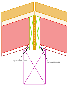
Detail First Mst. 1:10
