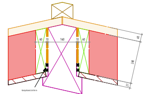
Detail Grat Mst. 1:10
